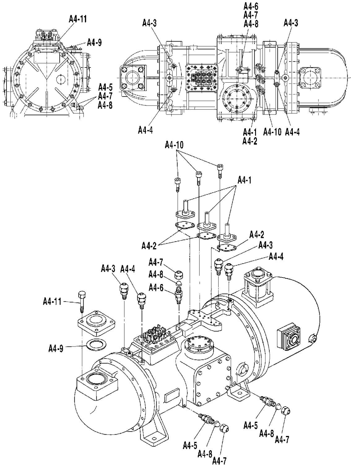
A4 Accessories diagram
