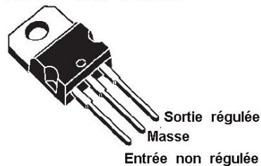
TO-220
