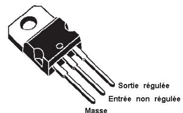
TO-220
