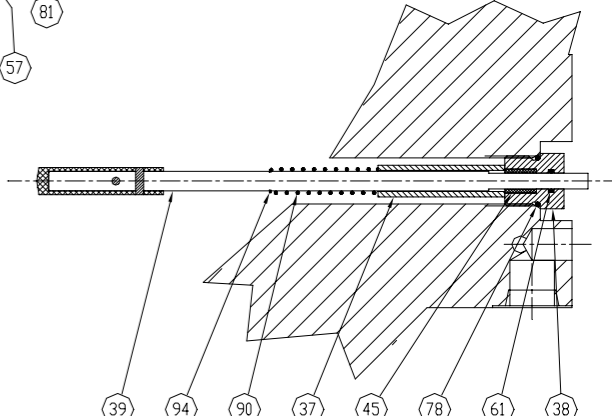
SECTION A-A FULL SCALE
