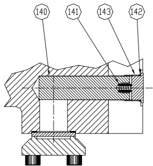
VIEW SHOWING ECONOMIZER PORT PLUGGED
